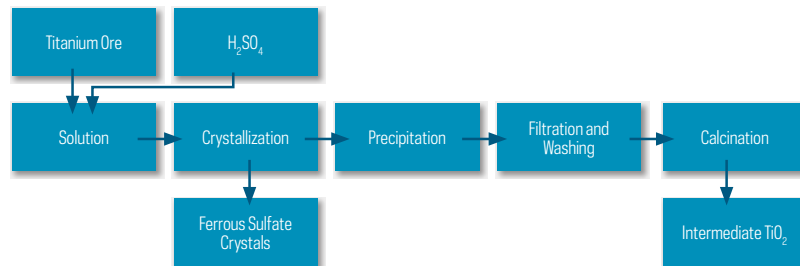
Figure 19 TiO 2 Manufacturing Processes
